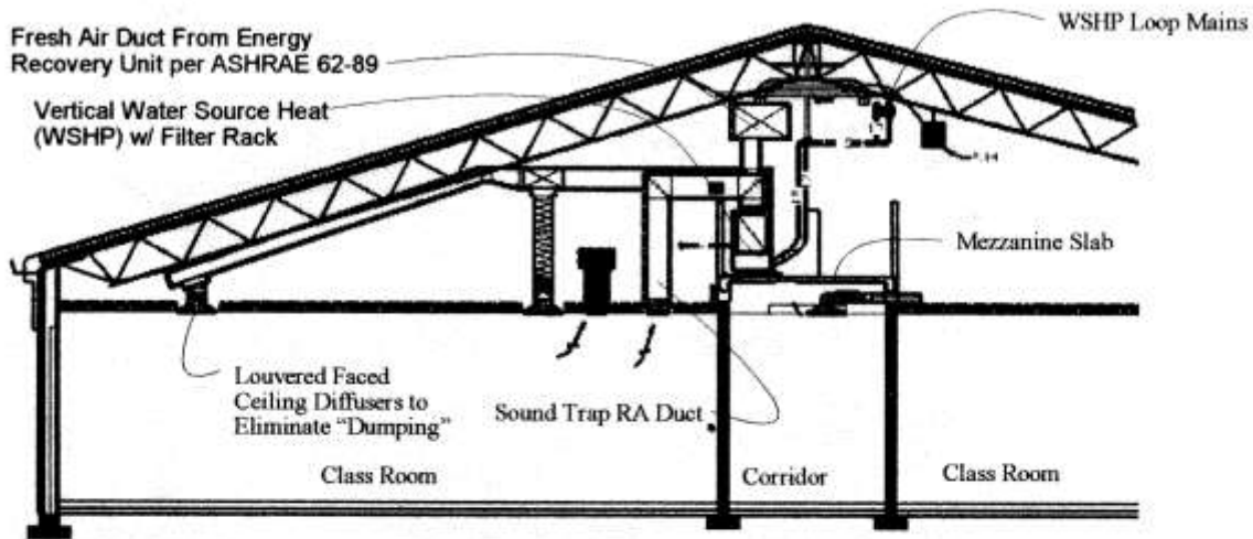
MEZZANINE SECTION THRU CLASSROOMS SCALE: _____ NONE
